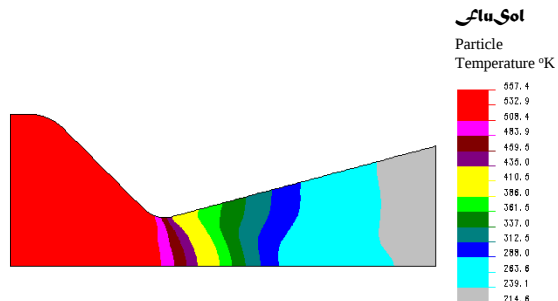
Particle temperature contour for mixture of solid particles and gas flow through a convergent divergent nozzle. The solid particles have 1 μm in diameter.
