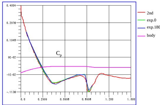
Cp distribution along the solid surface for Mach 1.6 flow past a circular-arc-cylinder-boattail projectile with Re=6.6 \times 10^6 .
