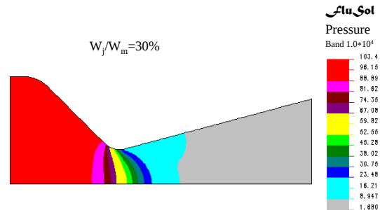
Gas pressure contour for mixture of solid particles and gas flow through a convergent-divergent nozzle. The solid particles have 1 μm in diameter.
