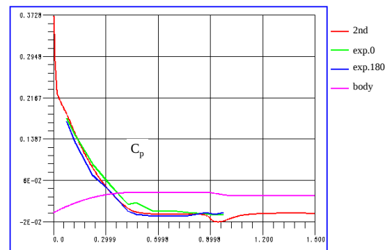
Cp distribution along the solid surface for Mach 4.63 flow past a circular-arc-cylinder-boattail projectile with Re=6.6 \times 10^6 .
