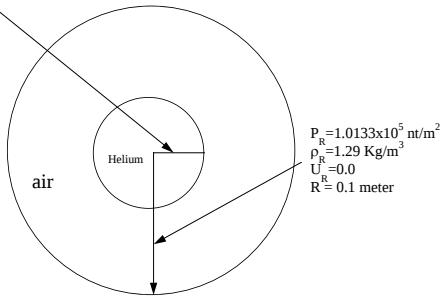
Computational domain for Helium spherically exploded into surrounded air.
