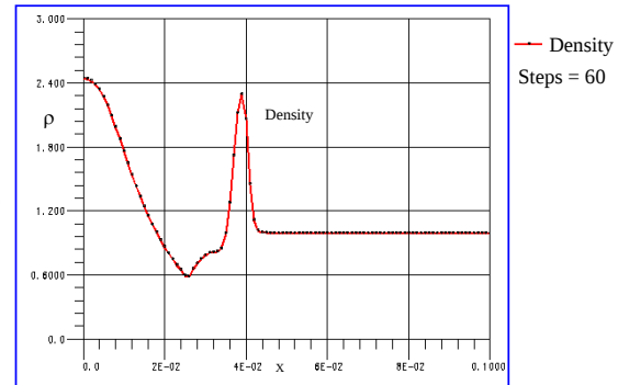
Density distribution at 60 time steps after the Helium sphere was broken.
