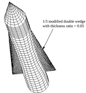
Step 3. Sweep 2D mesh around the axis line and create 3D mesh.
