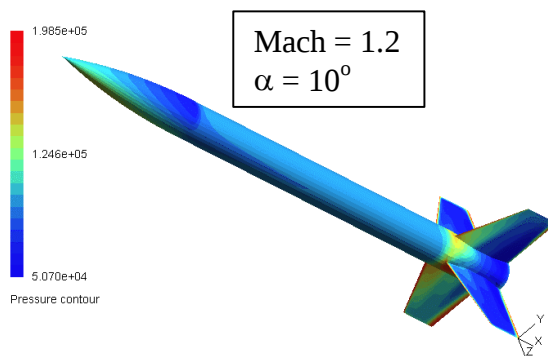
Pressure contour
