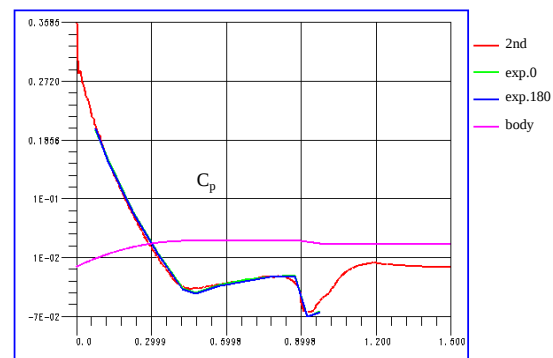
Cp distribution along the solid surface for Mach 2.3 flow past a circular-arc-cylinder-boattail projectile with Re=6.6 \times 10^6 .
