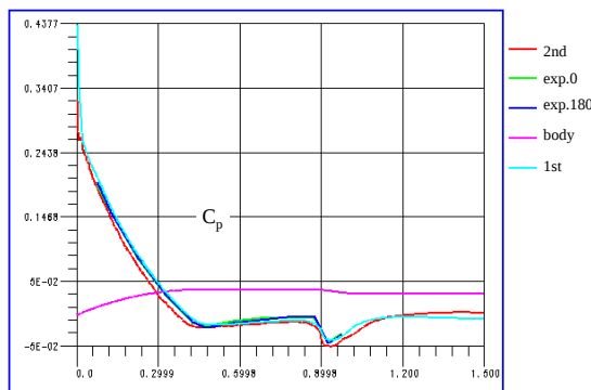
Cp distribution along the solid surface for Mach 2.96 flow past a circular-arc-cylinder-boattail projectile with Re=6.6 \times 10^6 .
