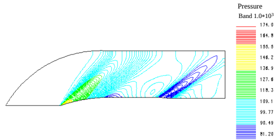
Pressure contour lines for Mach 1.6 flow past a circular-arc-cylinder-boattail projectile with Re=6.6 \times 10^6 .
