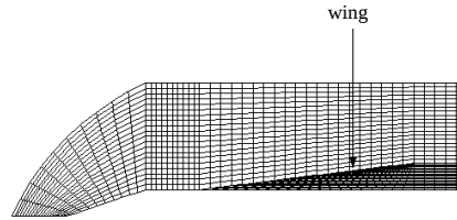
Step 2. Create 2D finite element mesh for wing-body combination. The shape of wing section and total number of wing to be created are also specified.
