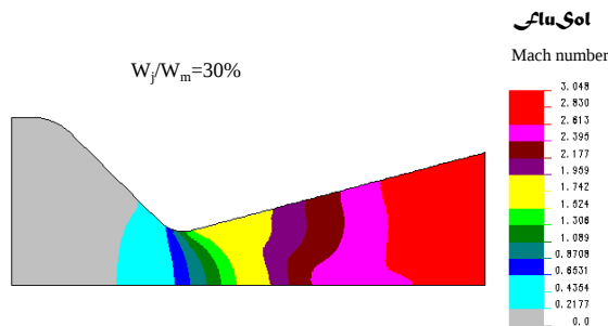
Gas Mach number contour for mixtures of solid particles and gas flow through a convergent divergent nozzle. The solid particles have 1 μm in diameter.
