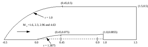
Supersonic flow past a circular-arc-cylinder-flare projectile.
