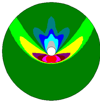
Cross sectional density contour for Mach 1.8 flow past a 5° cone at 45° angle of attack.
